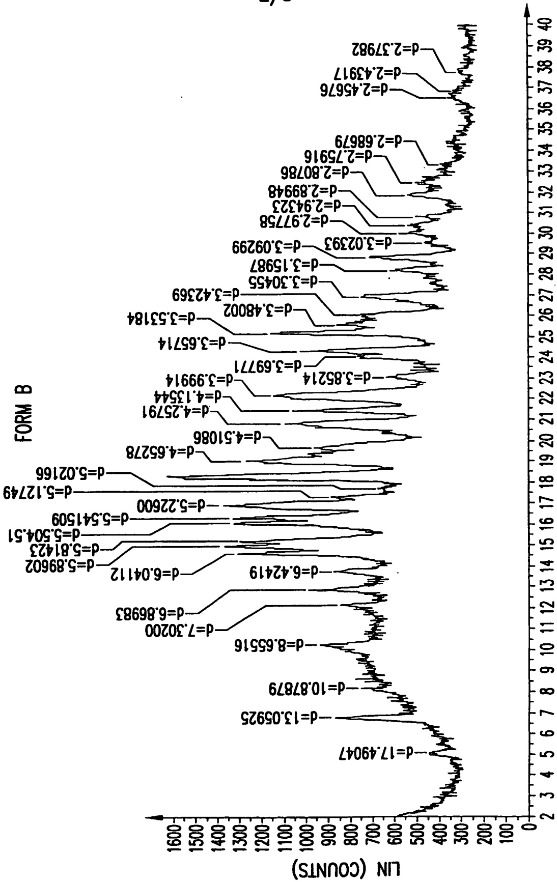
2-THETA - SCALE FIG.2
